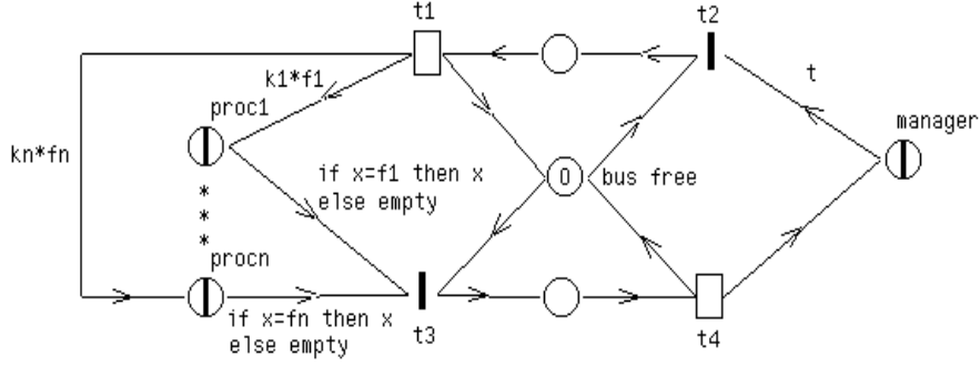
Fig. 2. QPN with k_i = (t \text{ div } n) + g(i, n, t) and g(i, n, t) := 1 if i \leq t \text{ mod } n and 0 else. compute the solution vector with an estimated accuracy of 0.01% including the times to generate state spaces and matrices from the model specification for the conventional approach. Columns 5 and 6 include the corresponding quantities for the hierarchical approach. For the conventional analysis immediate transitions are eliminated on net level. The last three columns of the table show the number of states, non-zero elements in the submatrices and analysis time for a reduced MC resulting from an exploitation of the identities of processors. The technique used for reduction has been introduced in [Bu3]. The largest MC which can be generated and analyzed with the conventional approach results from the model with t = 9 , for t = 10 we were not even able to generate the state space in an acceptable amount of time (i.e. less than 24 hours). With the new approach we can analyze the model for t = 13 which results in a MC with a state space twenty times larger than the one to be analyzable with conventional techniques. Additionally the new approach is faster for large models since paging is not necessary. Exploitation of symmetries yields a significant increase in the size of models which are solvable. Combining this reduction with the new analysis technique allows us to analyze models with t up to 20 which results in a MC about 3 orders of a magnitude larger than the MC solvable with the conventional approach.
