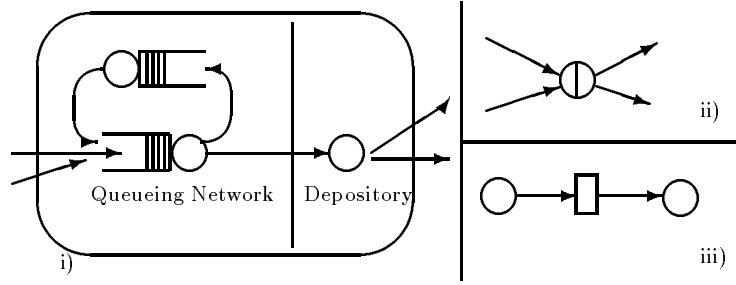
Fig. 1. i) Example timed queueing place of a QPN, ii) its pictorial representation, and iii) its simplified interpretation from a Petri Net point of view
